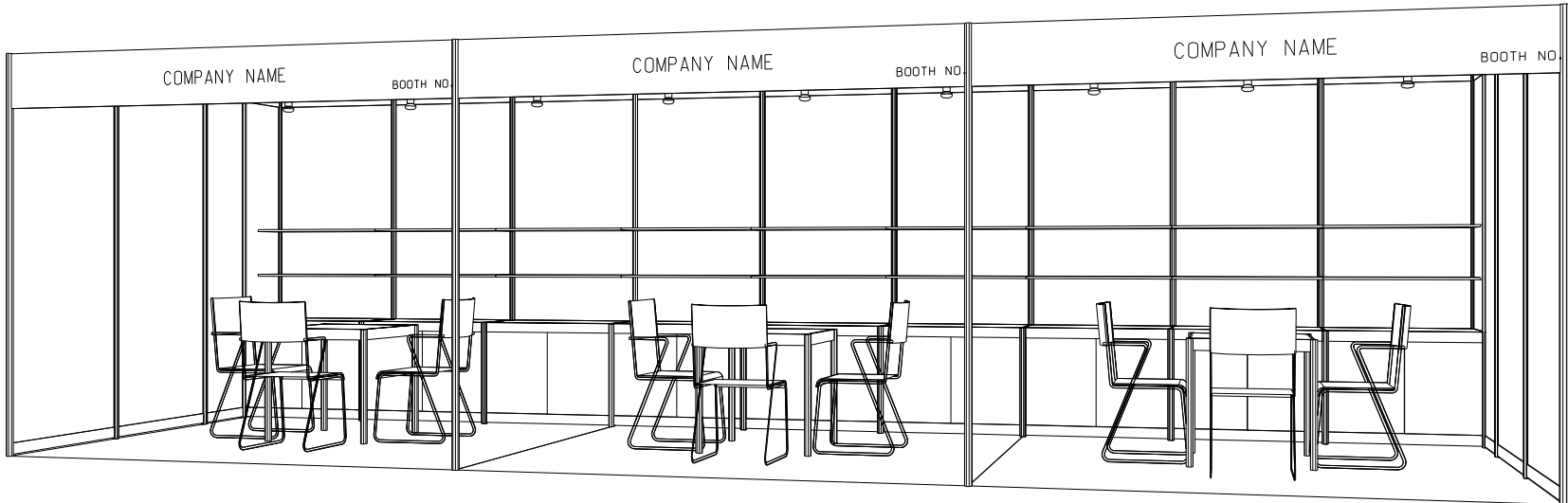
PERSPECTIVE 9M(W) X 3M(D) X 2.5M(H) Standard Booth A
